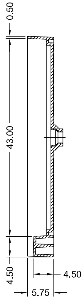
SECTION B-B
